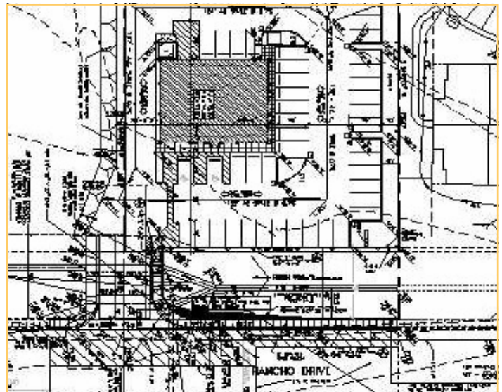
Prototype grading plan for one of CivilWorksInc's many projects in Las Vegas, Nevada.
